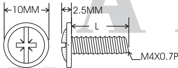
SCREW
